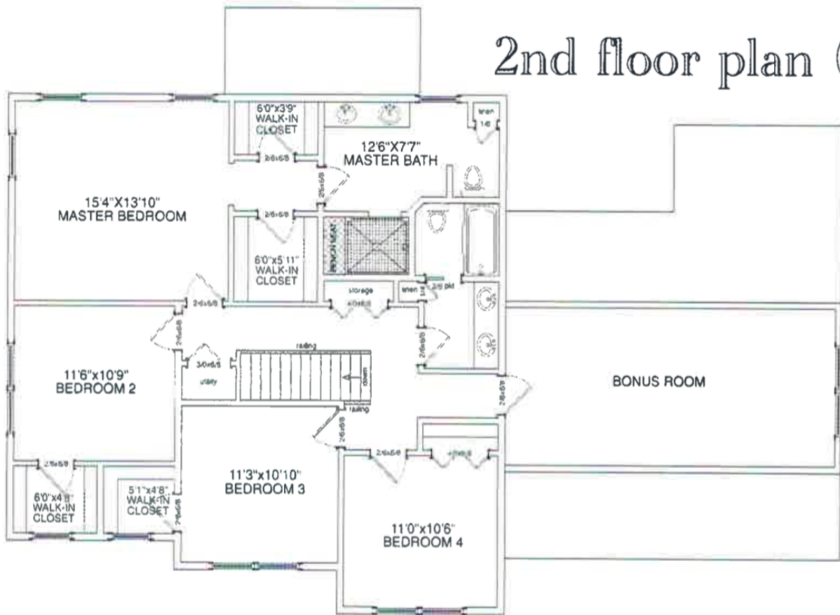
2nd floor plan (b)
